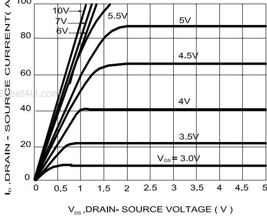
ON-REGION CHARACTERISTIC
