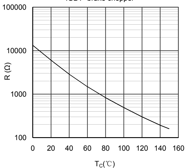
Figure 14. NTC Characteristics
