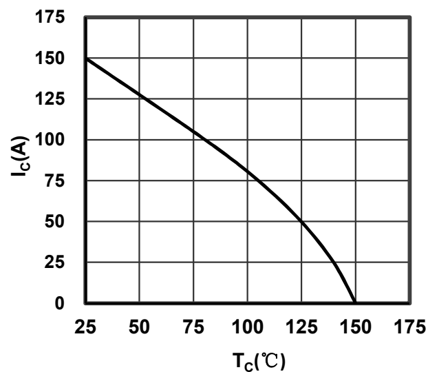
Figure 7. Collector Current vs Case temperature
