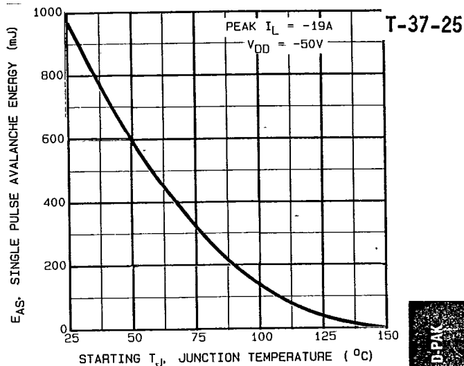
Fig. 14c — Maximum Avalanche Vs. Starting Junction Temperature
