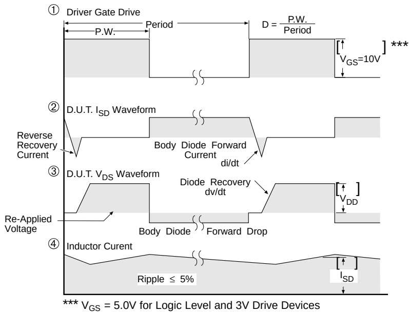
Fig 14. For P-Channel HEXFETS
