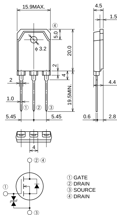
OUTLINE DRAWING
