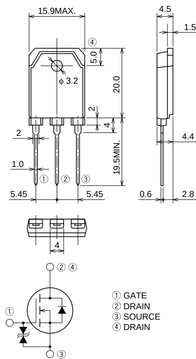
OUTLINE DRAWING
