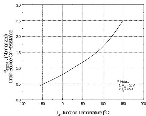
Figure 8. On-Resistance Variation
