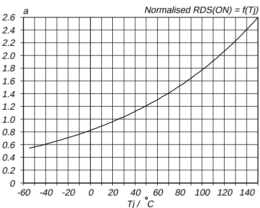
Fig.9. Normalised drain-source on-state resistance. a = R_{DS(ON)} / R_{DS(ON)25^\circ\text{C}} = f(T_j) ; I_D = 1.5 \text{ A} ; V_{GS} = 10 \text{ V}
