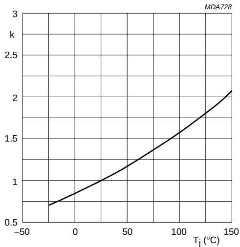
Fig.8 k = \frac{R_{DS(on)} \text{ at } T_j}{R_{DS(on)} \text{ at } 25\text{ }^\circ\text{C}}; typ. values at 500 mA/10 V.
