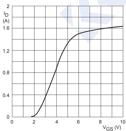
Fig.6 Transfer characteristic; V_{DS} = 10\text{ V} ; T_j = 25^\circ\text{C} ; typical value.
