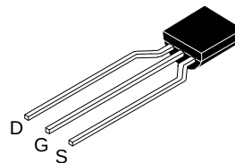
TO-92 3 4.83x4.76 LEADFORMED CASE 135AR
