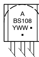
TO-92 CASE 29-11 STYLE 30
