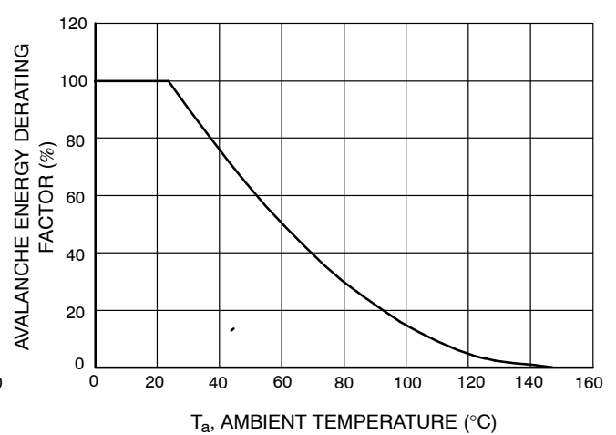
Figure 15. E_{AS} - T_a
