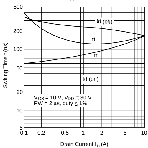
Switching Characteristics
