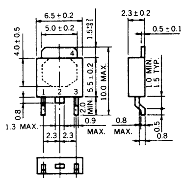
2SK1059-Z
