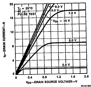
Figure 1 Output Characteristics
