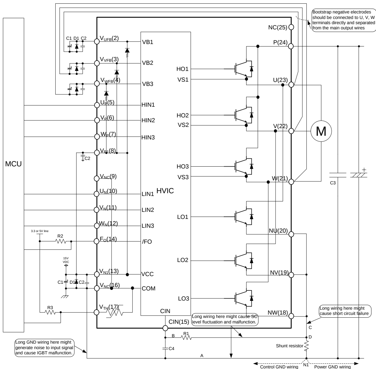
Typical Application Circuit
