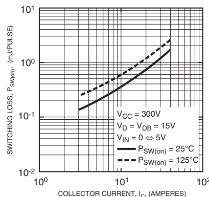
SWITCHING LOSS (ON) VS. COLLECTOR CURRENT (TYPICAL - P-SIDE)
