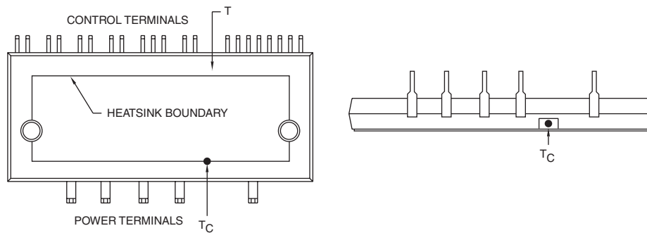
T_C Measurement Point
