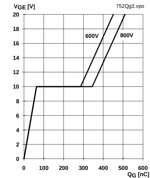
Fig. 13 Typ. gate charge characteristic
