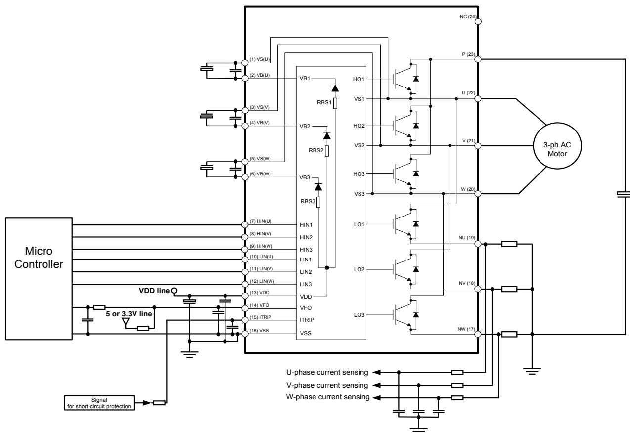
Figure 8: Application circuit
