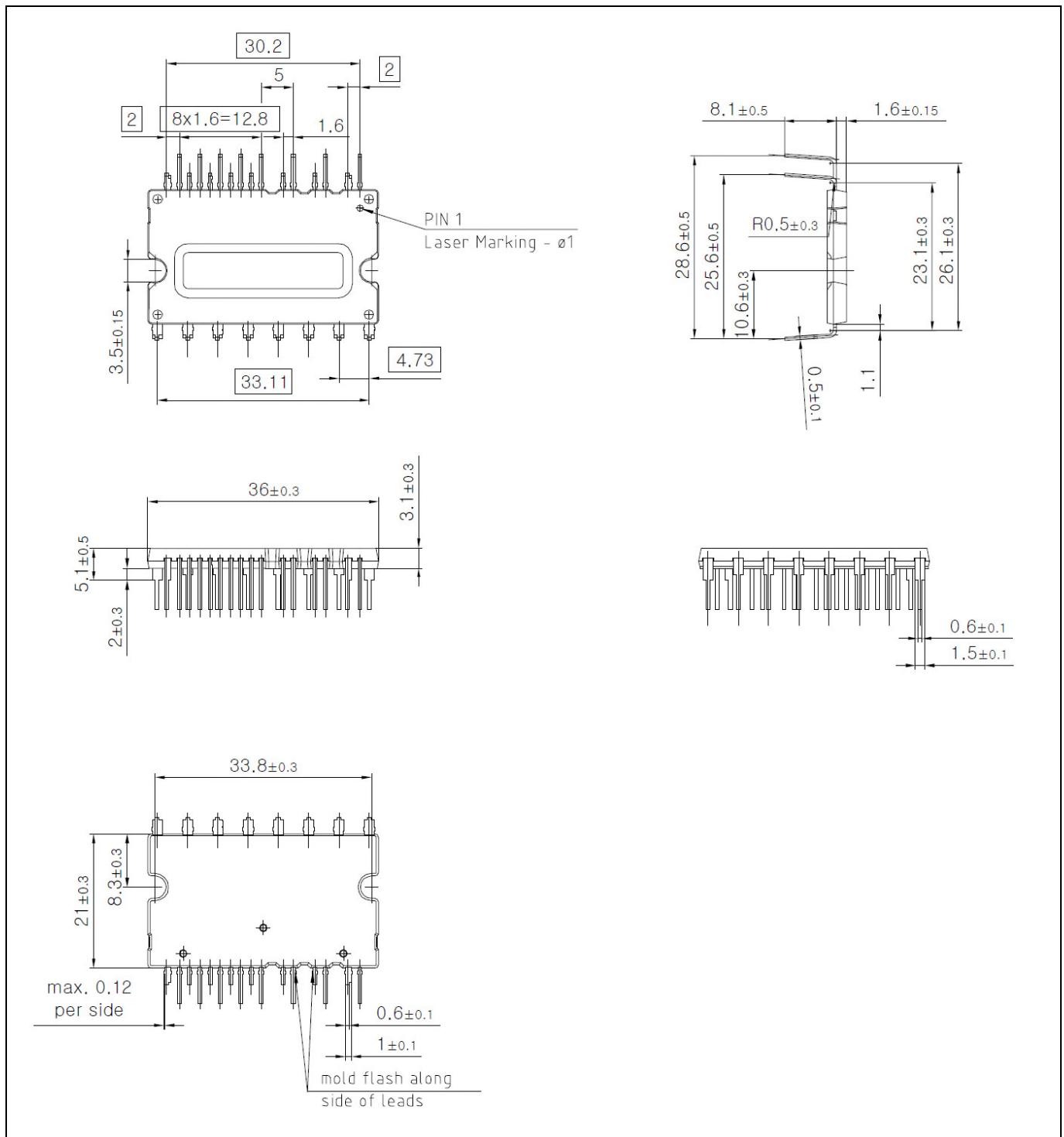
Figure 12 IGCM15F60GA
