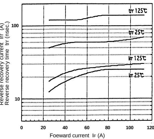
Reverse recovery characteristics t_{rr} , I_{rr} , vs. I_F
